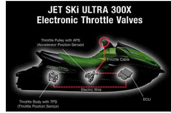
Electronic throttle valves
